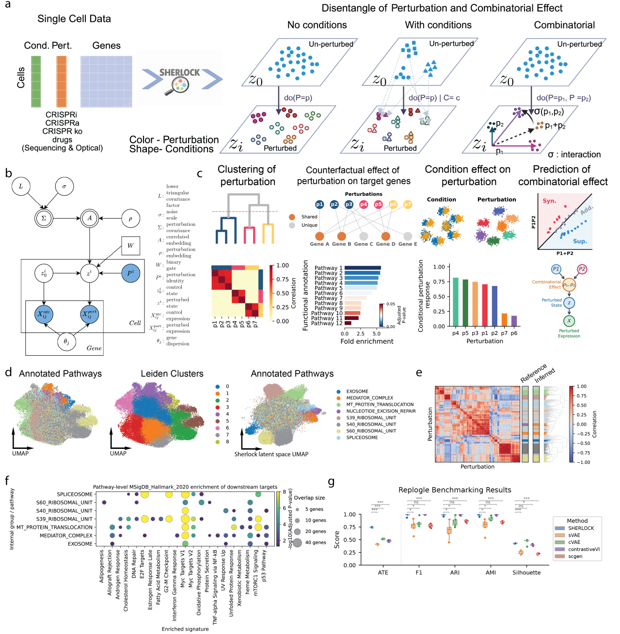
Figure 1: SHERLOCK: a generative framework for disentangling perturbation effects in single-cell data. (a) Overview of SHERLOCK. Single-cell gene expression data, together with perturbation and condition labels, are modeled using a structured variational autoencoder (VAE) to disentangle perturbation effects, context-dependent responses, and combinatorial interactions. (b) Plate diagram of the SHERLOCK generative process. Uncolored circles denote inferred variables, colored circles denote observed variables, and squares denote observed constants. (c) Main functionalities of SHERLOCK. (d) Left: UMAP of the original gene expression space from the Replogle dataset, colored by pathway-level annotations. Middle: UMAP of the original gene expression space, colored by Leiden clusters. Right: SHERLOCK latent representation of the same cells, colored by pathway-level annotations. (e) Correlation matrix of the learned perturbation embedding. Reference pathway annotations were annotated by Replogle et al., whereas mapped pathways were inferred from SHERLOCK groupings. (f) Gene set enrichment analysis (GSEA) of the inferred downstream target genes for each perturbation group, highlighting pathway-relevant functional signatures. Color indicates -\log_{10} -transformed adjusted p -values, and point size represents the number of overlapping genes between the inferred target genes and enriched pathways. (g) Benchmarking of SHERLOCK on the Replogle dataset. ATE: average treatment effect; ARI: adjusted Rand index; AMI: adjusted mutual information.
