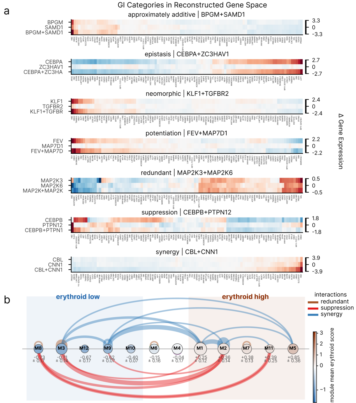
Figure 5: Genetic interaction classes reveal distinct transcriptional effects and lineage-associated module relationships. (a) Reconstructed responses to the two constituent single perturbations and their combination for a representative pair per interaction category (100 highest-variance genes). (b) Each labeled pair is drawn as an arc between the consensus modules of its two parents. Modules run from erythroid low on the left to erythroid high on the right, with their mean observed erythroid score and its standard error over member perturbations printed below each one; node color repeats that score (color bar) and node size scales with the number of members. Arc color indicates the interaction class including redundant, suppression, and synergy.
