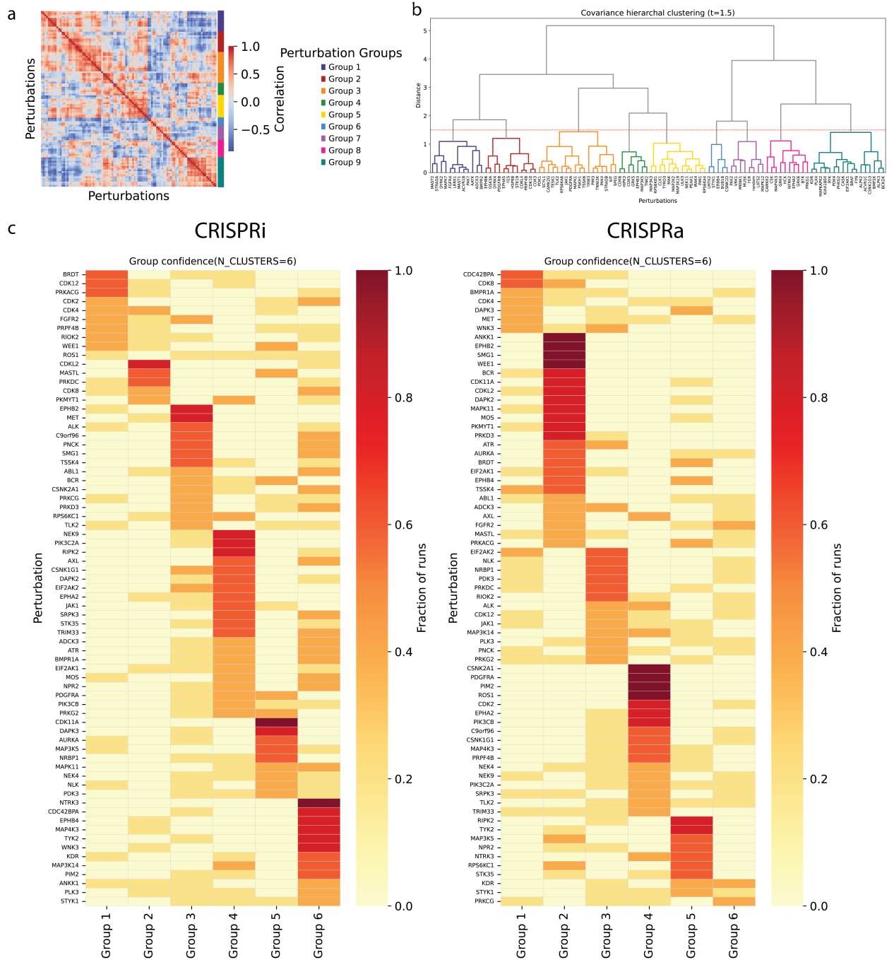
Figure S3: Robust and reproducible clustering of kinase perturbations across SHERLOCK runs. (a) Perturbation correlations derived from posterior row-covariance matrix ( \Sigma_p ) of perturbation embeddings from the CRISPRa drug-target screen, revealing pathway-level block structure among genetic perturbations. (b) Hierarchical clustering of CRISPRa perturbation embeddings identifies coherent groups of functionally related genes, consistent with the covariance-based organization learned by SHERLOCK. c, Cluster assignment confidence across repeated SHERLOCK runs for CRISPR interference (CRISPRi; left) and CRISPR activation (CRISPRa; right). Each row represents a kinase perturbation, and each column represents one of the six consensus groups. Color intensity denotes the fraction of independent SHERLOCK runs in which a perturbation was assigned to each group, demonstrating reproducible clustering across both perturbation modalities.
