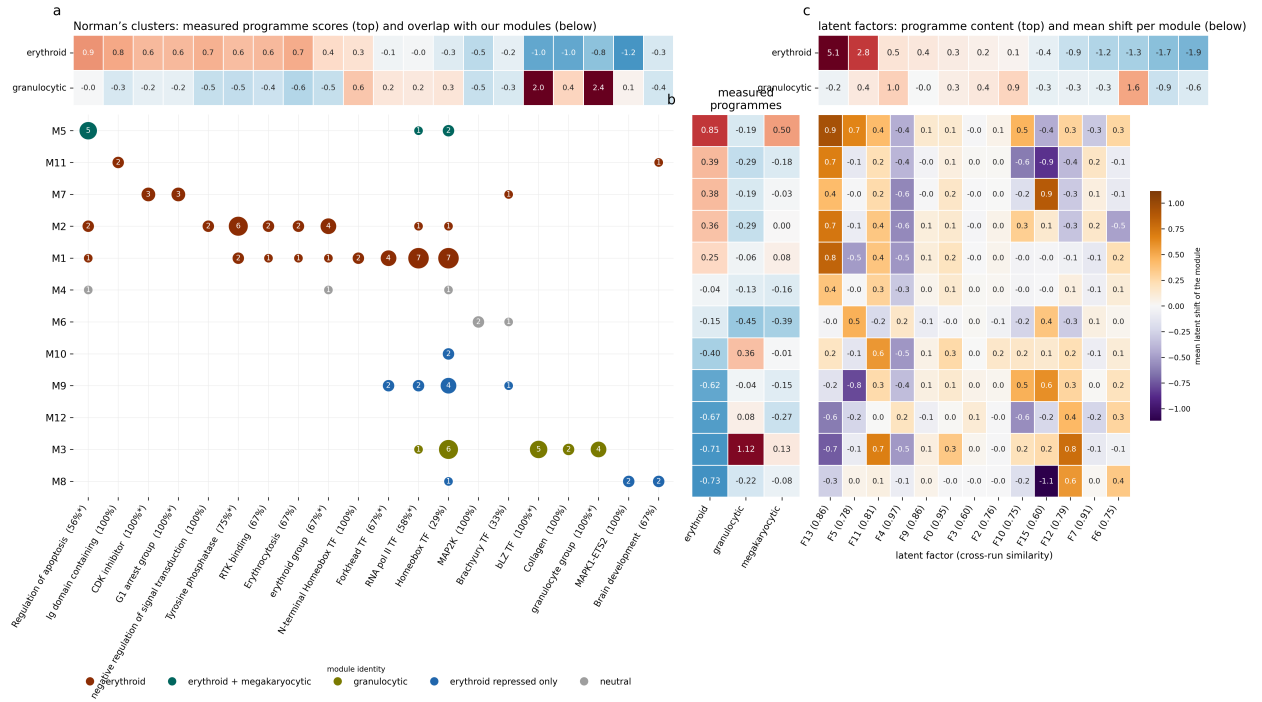
Figure S12: Consensus modules against Norman's clusters, measured programs and latent factors. (a) Overlap between the consensus modules (rows) and Norman et al.'s perturbation-map clusters and phenotype groups (columns); dot size and number give the members shared, dot color the module's identity, and the percentage under each cluster the share of its members in its best module (asterisk, BH q < 0.05 against random modules of the same sizes). The strip above gives each cluster's own measured erythroid and granulocytic scores. (b) Mean measured erythroid, granulocytic and megakaryocytic scores per module. The megakaryocytic score is a weak signal: scoring independent halves of each perturbation's cells agrees at 0.84, against 0.99 and 0.97 for the other two lineages. (c) Mean shift of each perturbation module along each reproducible latent factor, with the strip above giving each factor's erythroid and granulocytic content; factors are labeled with their cross-run signature similarity in parentheses.
